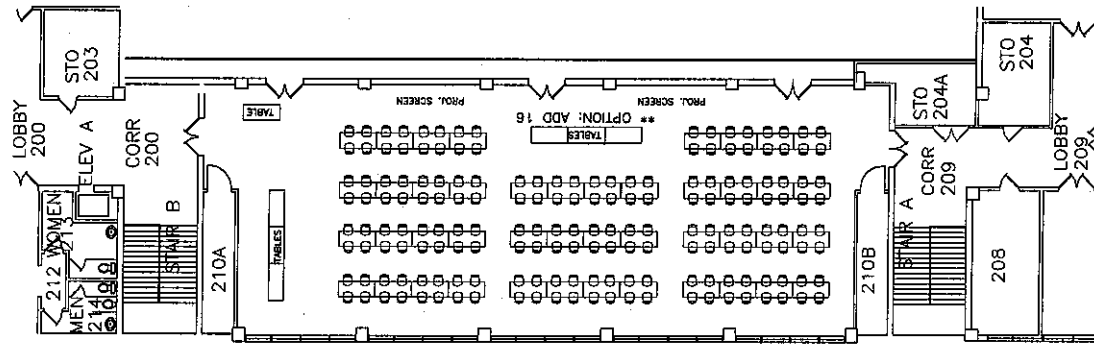
SCANLAN ROOM LAYOUT #2 OCCUPANCY: 11@16=176 DINING (44 RECT. TABLES/176 CHAIRS + 7 MISC. RECT. TABLES.....) ** OPTION: ADD 16
